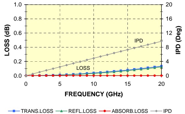
RAYDEL M26 RF PERFORMANCE AT NORMAL INCIDENCE
